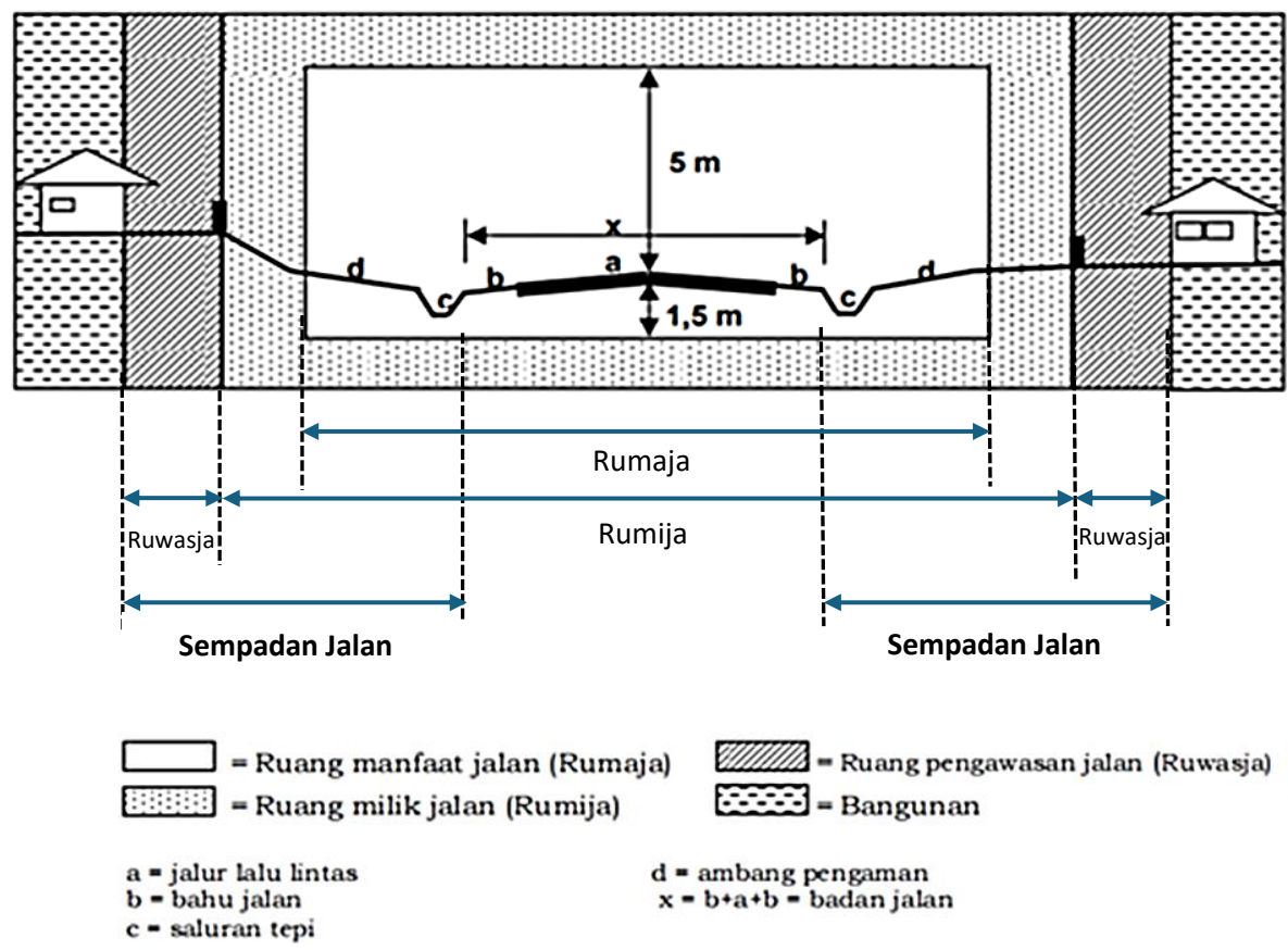
Penampang Bagian-bagian Jalan
